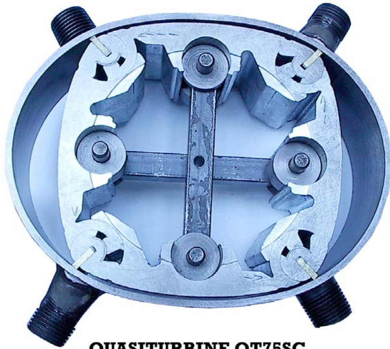
QUASITURBINE QT75SC
